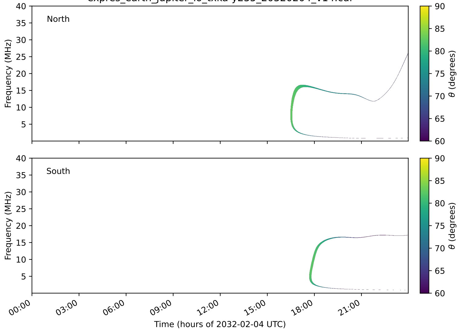
expres_earth_jupiter_io_txka-y235_20320204_v14.cdf
