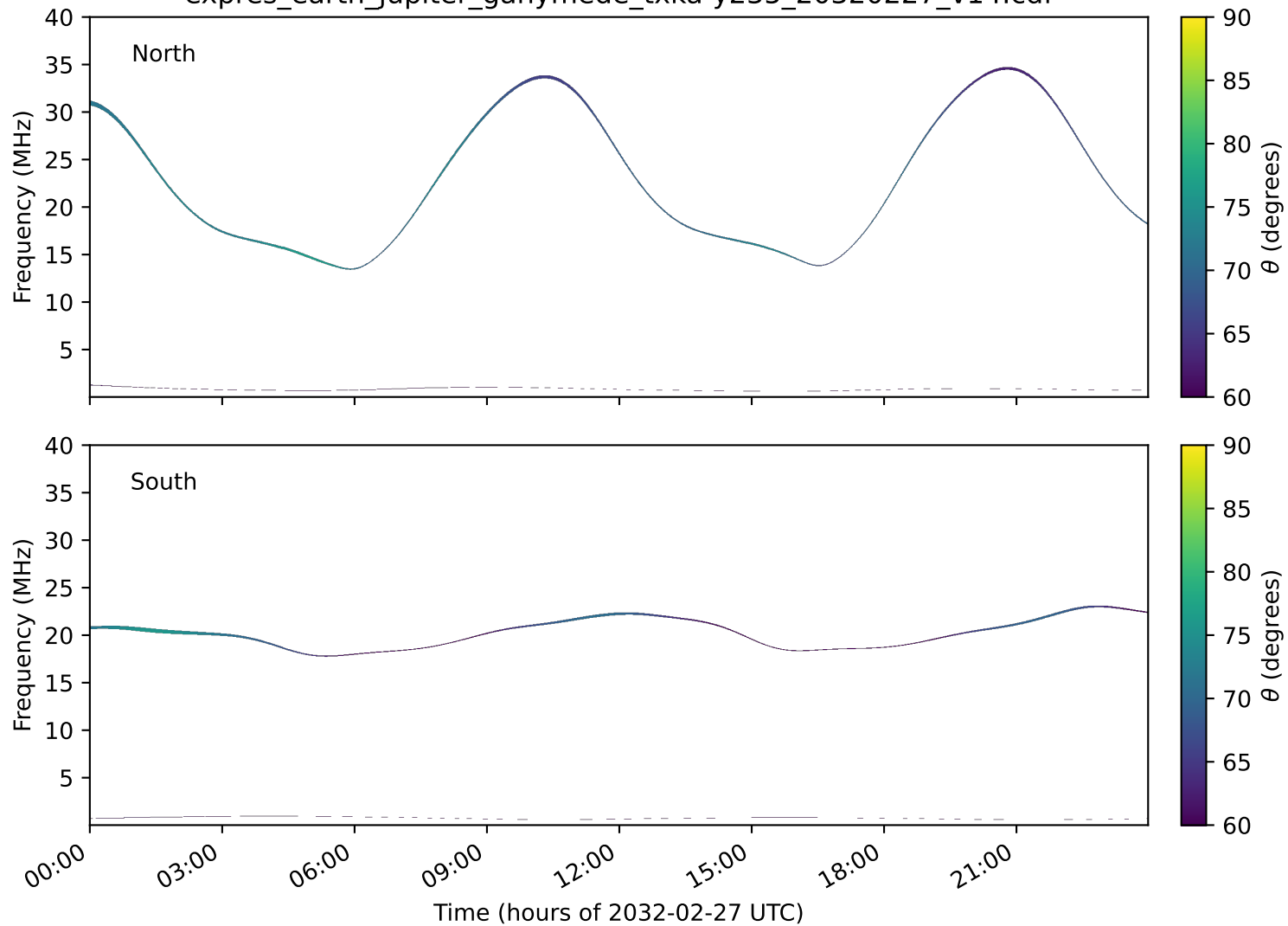
expres_earth_jupiter_ganymede_txka-y235_20320227_v14.cdf
