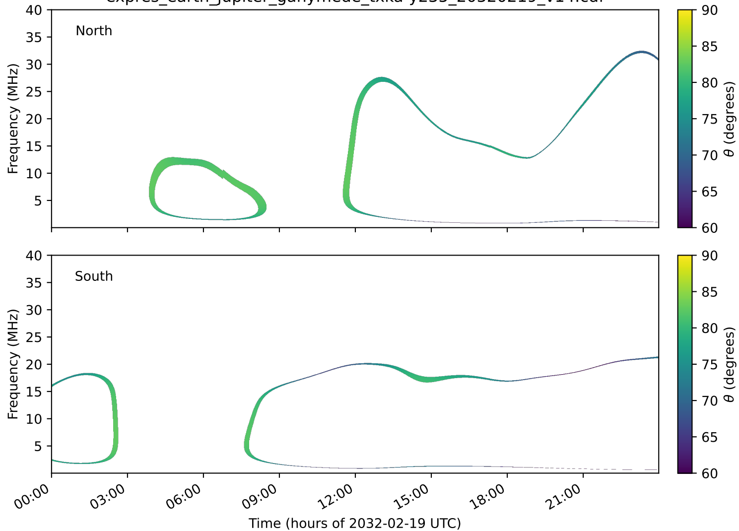
expres_earth_jupiter_ganymede_txka-y235_20320219_v14.cdf
