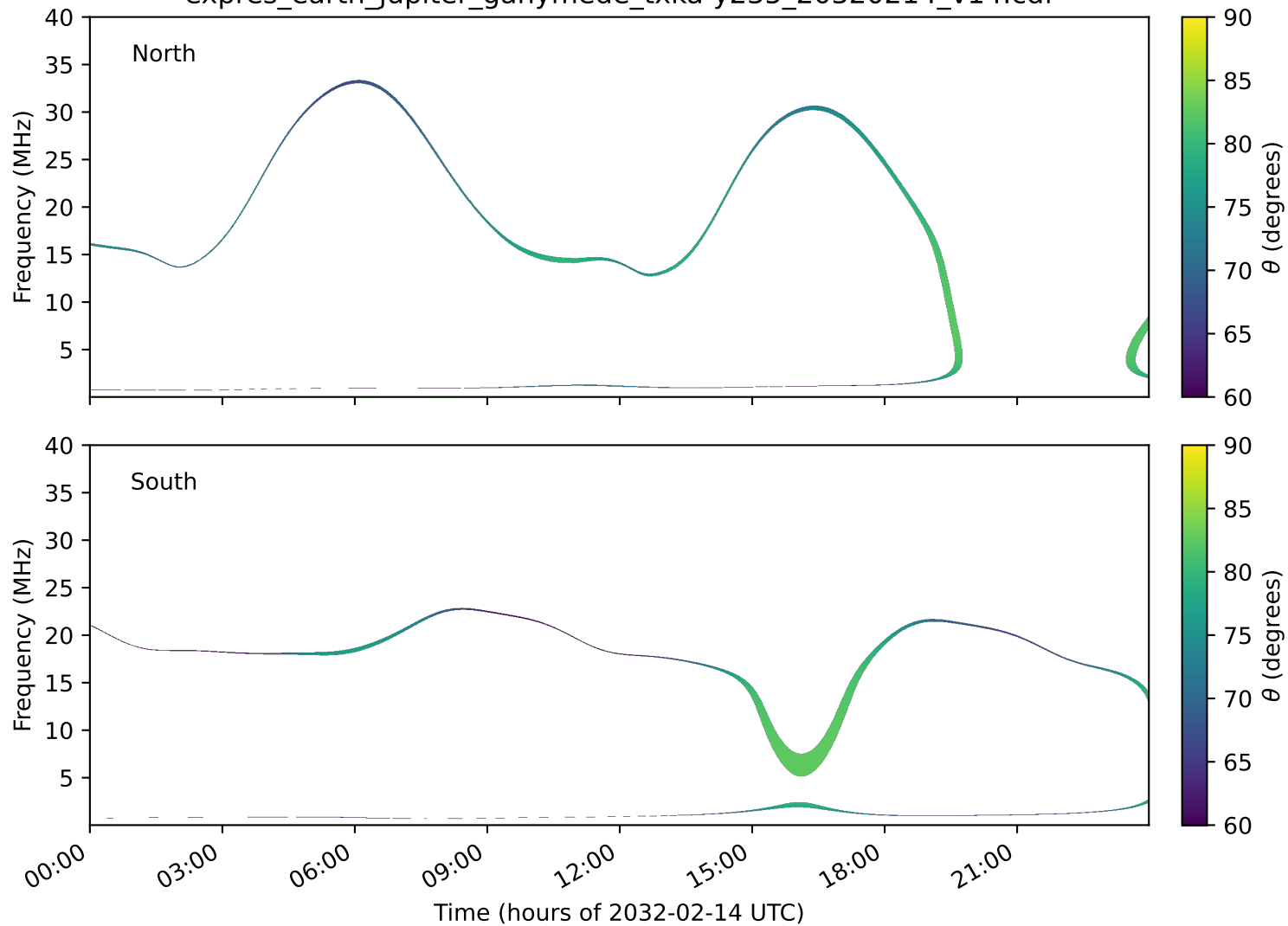
expres_earth_jupiter_ganymede_txka-y235_20320214_v14.cdf
