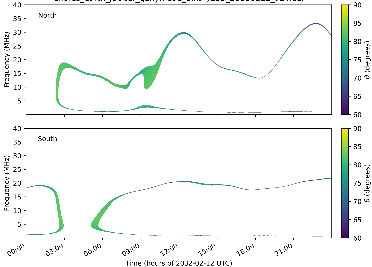
expres_earth_jupiter_ganymede_txka-y235_20320212_v14.cdf
