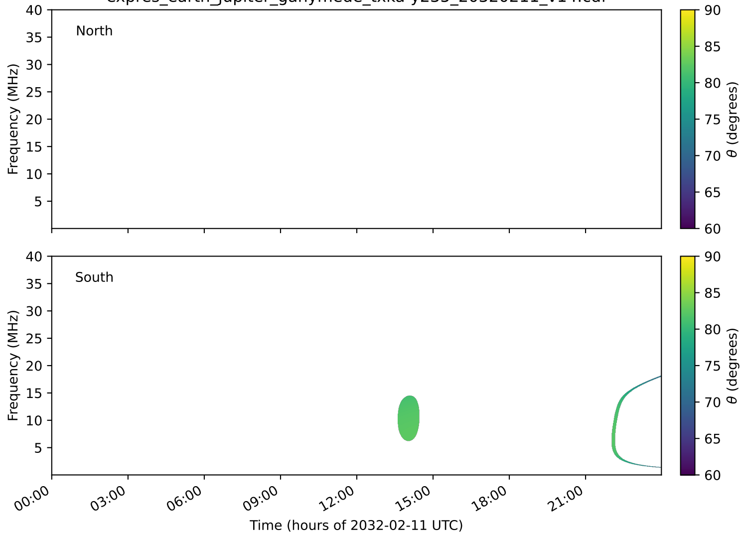
expres_earth_jupiter_ganymede_txka-y235_20320211_v14.cdf
