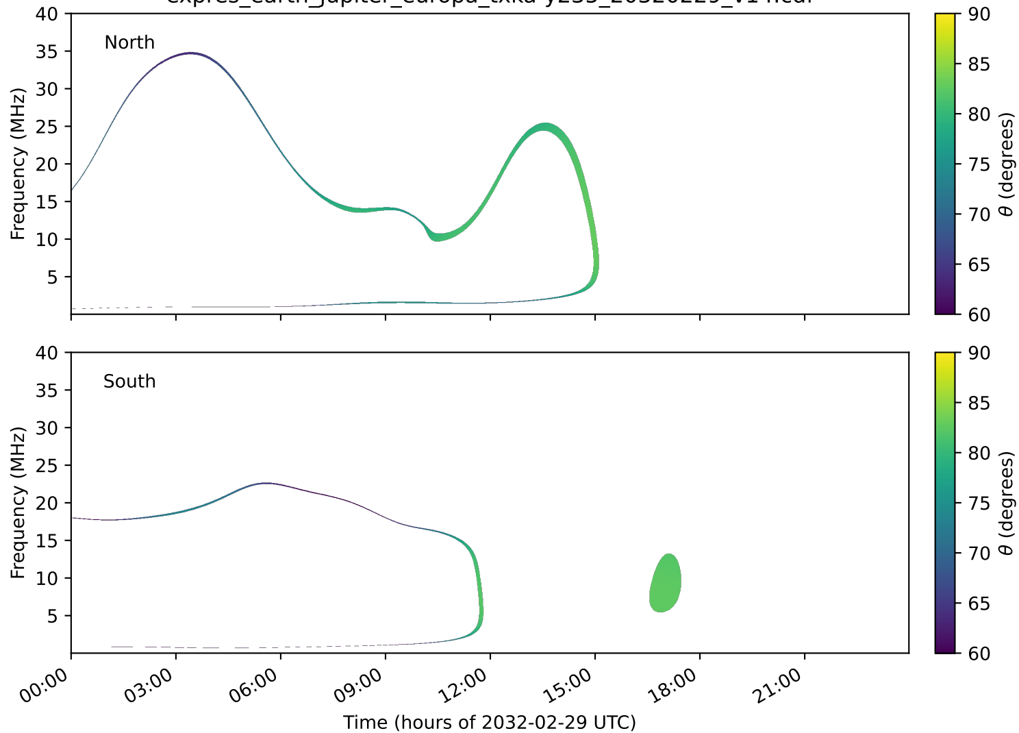
expres_earth_jupiter_europa_txka-y235_20320229_v14.cdf
