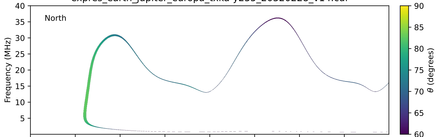
expres_earth_jupiter_europa_txka-y235_20320228_v14.cdf
