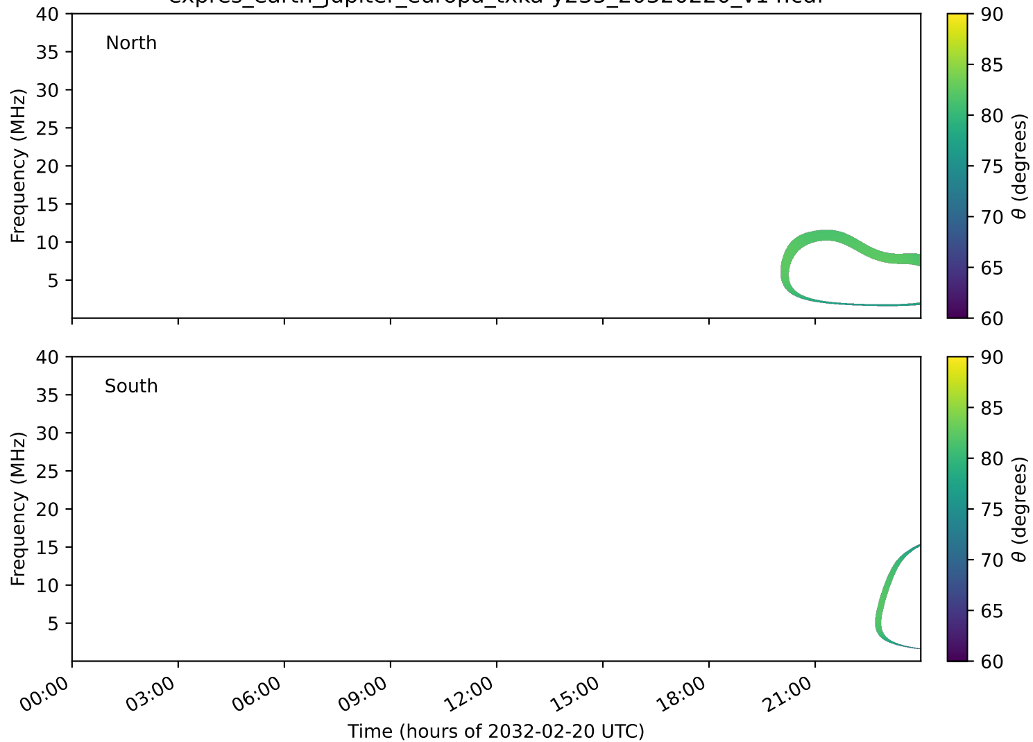
expres_earth_jupiter_europa_txka-y235_20320220_v14.cdf
