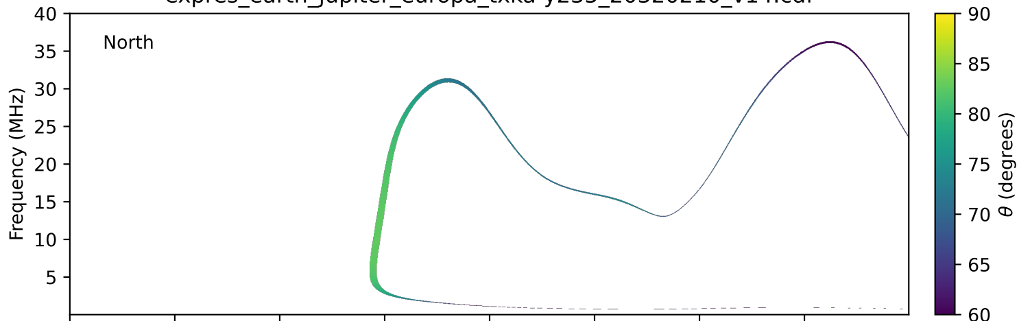
expres_earth_jupiter_europa_txka-y235_20320210_v14.cdf
