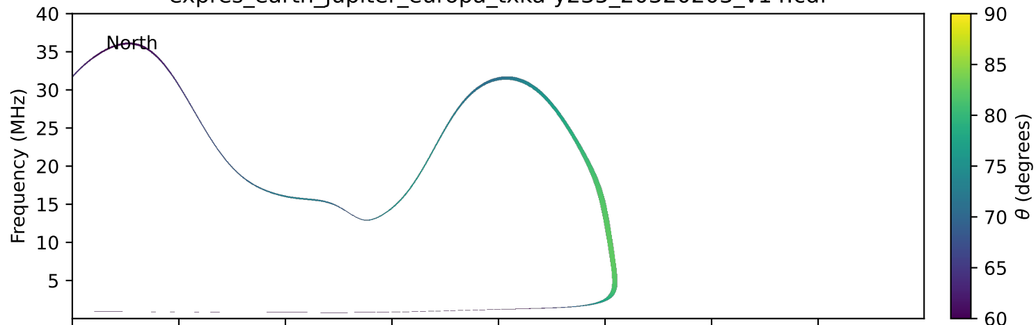
expres_earth_jupiter_europa_txka-y235_20320203_v14.cdf
