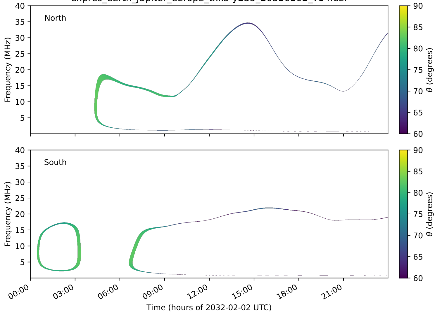
expres_earth_jupiter_europa_txka-y235_20320202_v14.cdf
