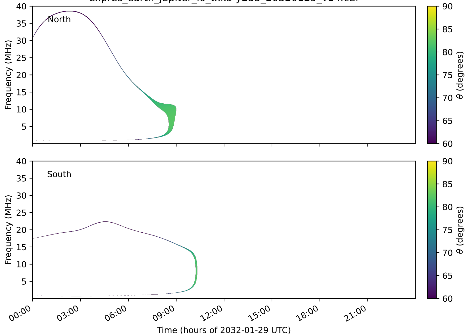
expres_earth_jupiter_io_txka-y235_20320129_v14.cdf
