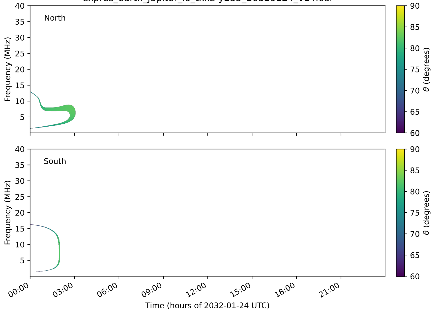
expres_earth_jupiter_io_txka-y235_20320124_v14.cdf
