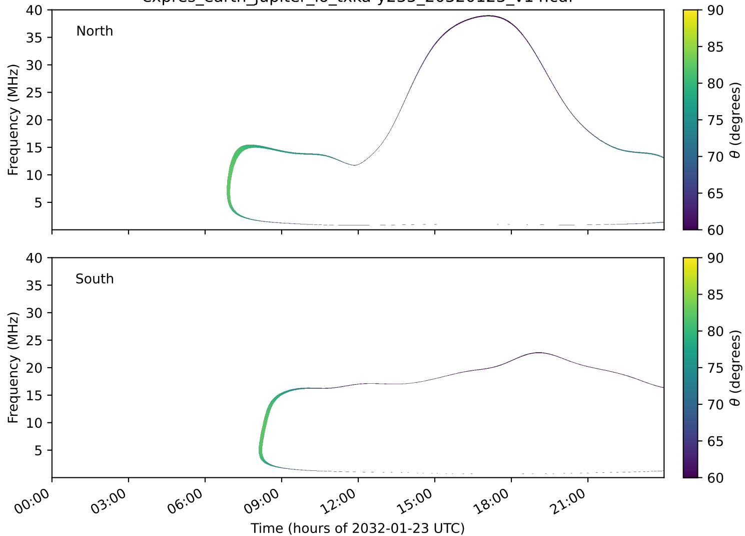
expres_earth_jupiter_io_txka-y235_20320123_v14.cdf
