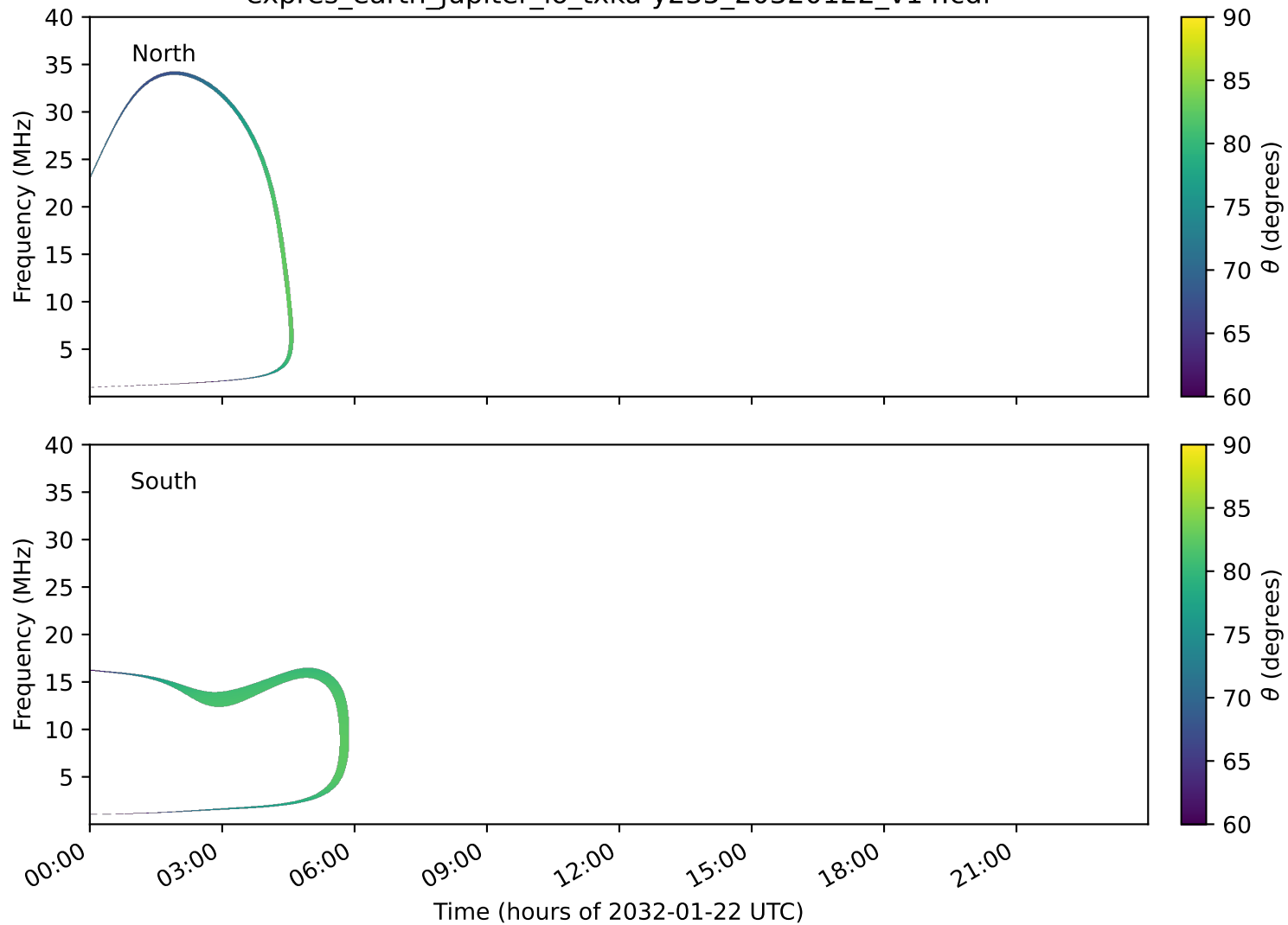
expres_earth_jupiter_io_txka-y235_20320122_v14.cdf
