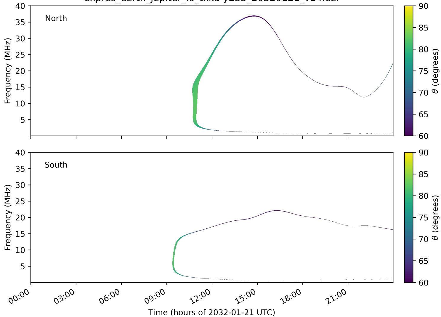
expres_earth_jupiter_io_txka-y235_20320121_v14.cdf
