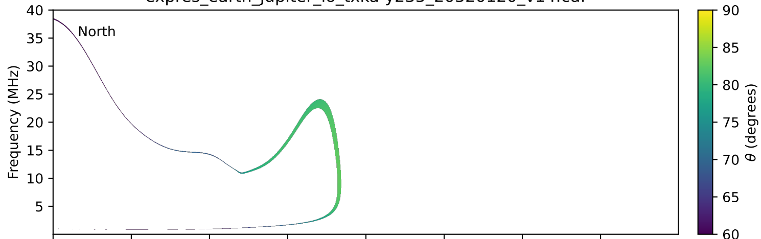
expres_earth_jupiter_io_txka-y235_20320120_v14.cdf
