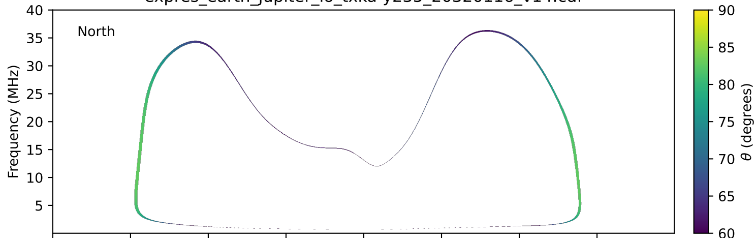
expres_earth_jupiter_io_txka-y235_20320116_v14.cdf
