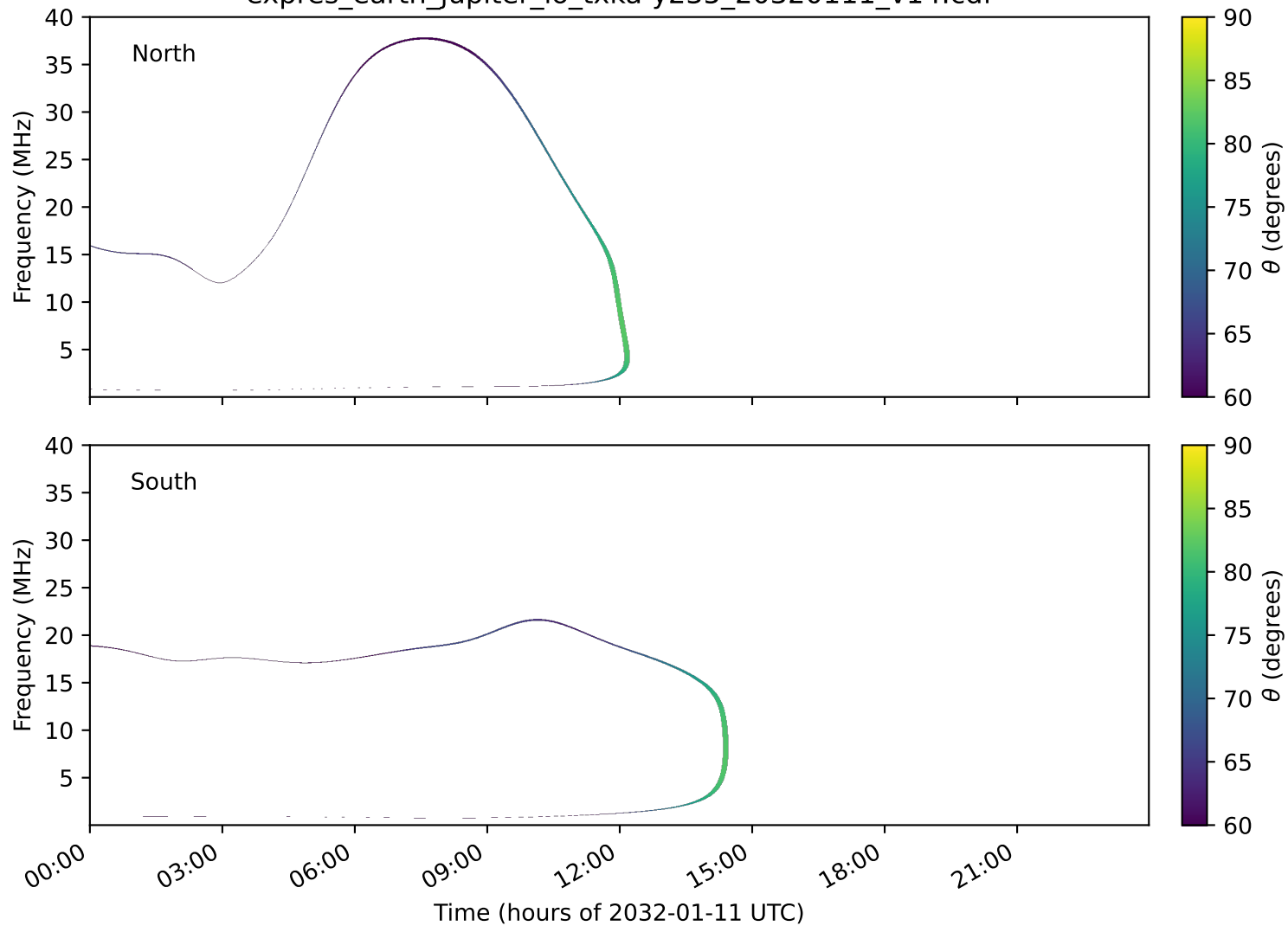
expres_earth_jupiter_io_txka-y235_20320111_v14.cdf
