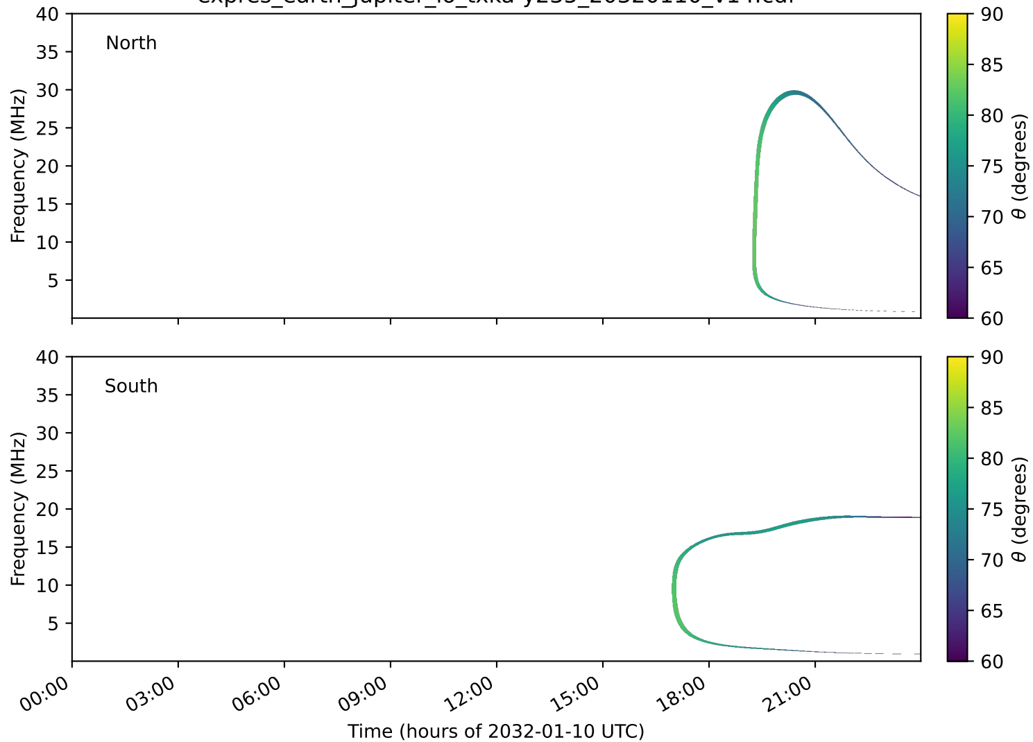
expres_earth_jupiter_io_txka-y235_20320110_v14.cdf
