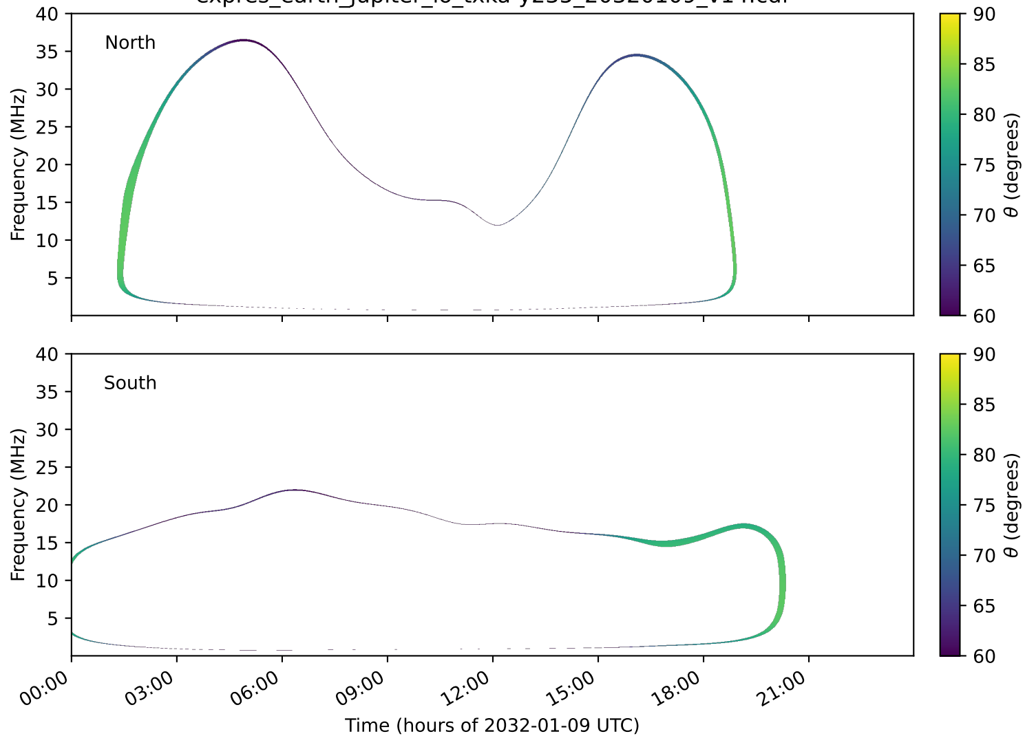
expres_earth_jupiter_io_txka-y235_20320109_v14.cdf
