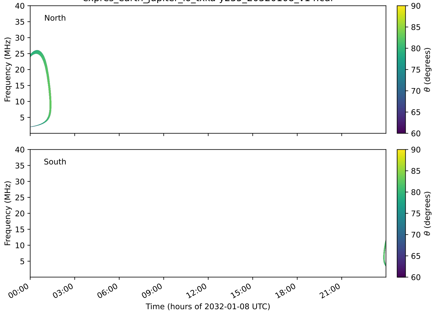
expres_earth_jupiter_io_txka-y235_20320108_v14.cdf
