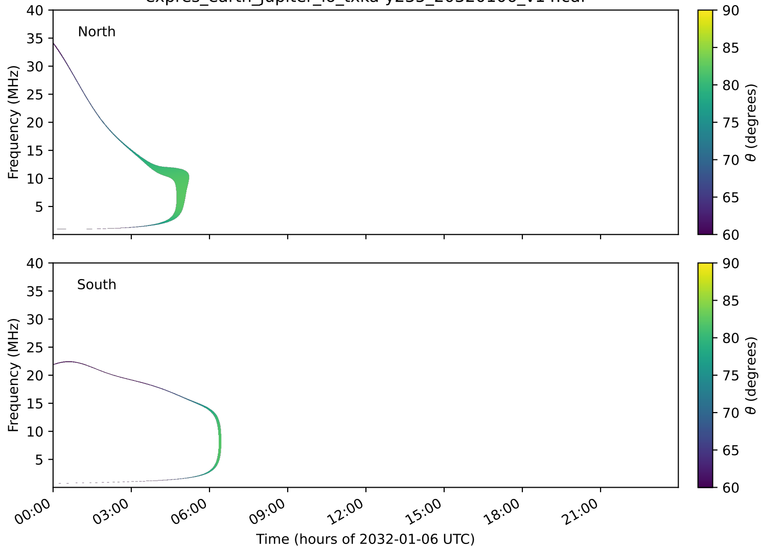
expres_earth_jupiter_io_txka-y235_20320106_v14.cdf
