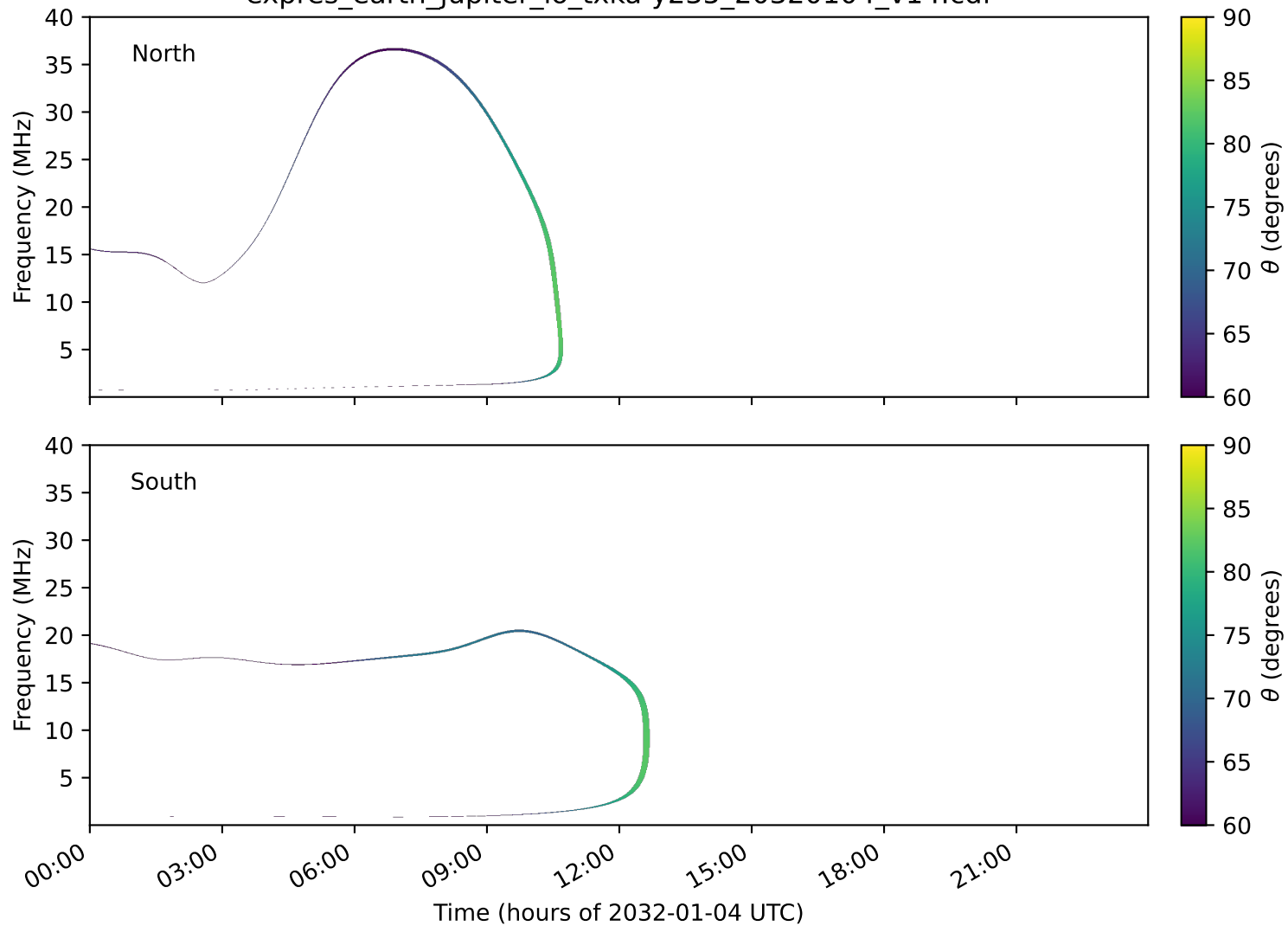
expres_earth_jupiter_io_txka-y235_20320104_v14.cdf
