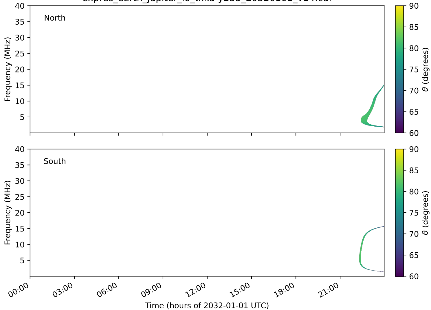
expres_earth_jupiter_io_txka-y235_20320101_v14.cdf
