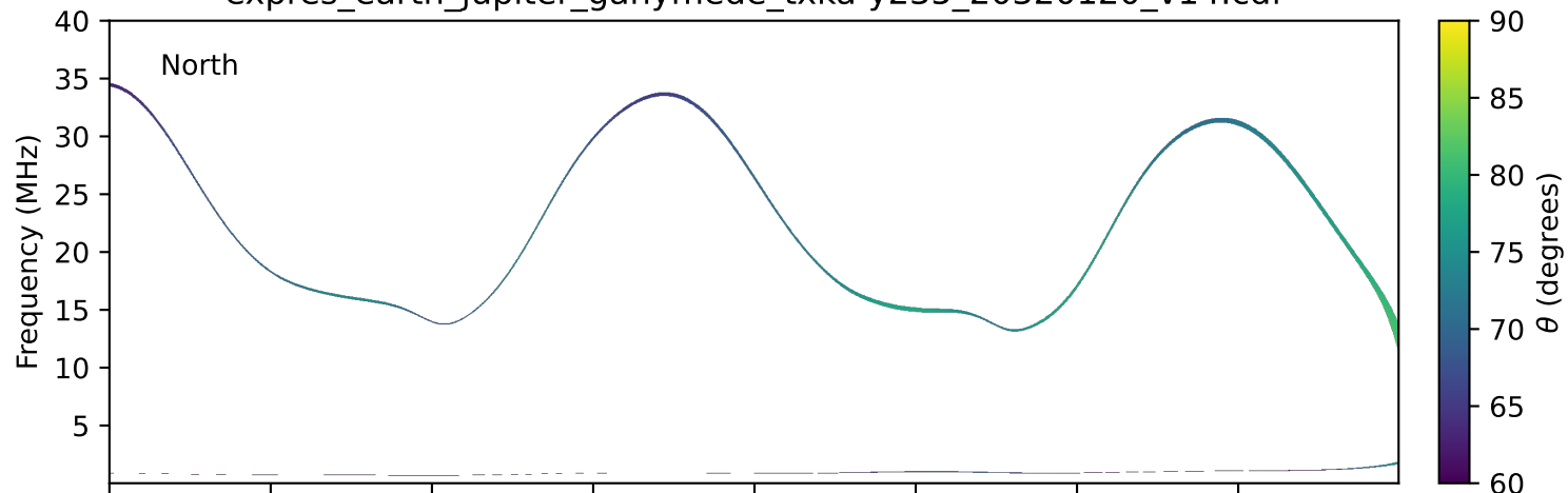
expres_earth_jupiter_ganymede_txka-y235_20320120_v14.cdf
