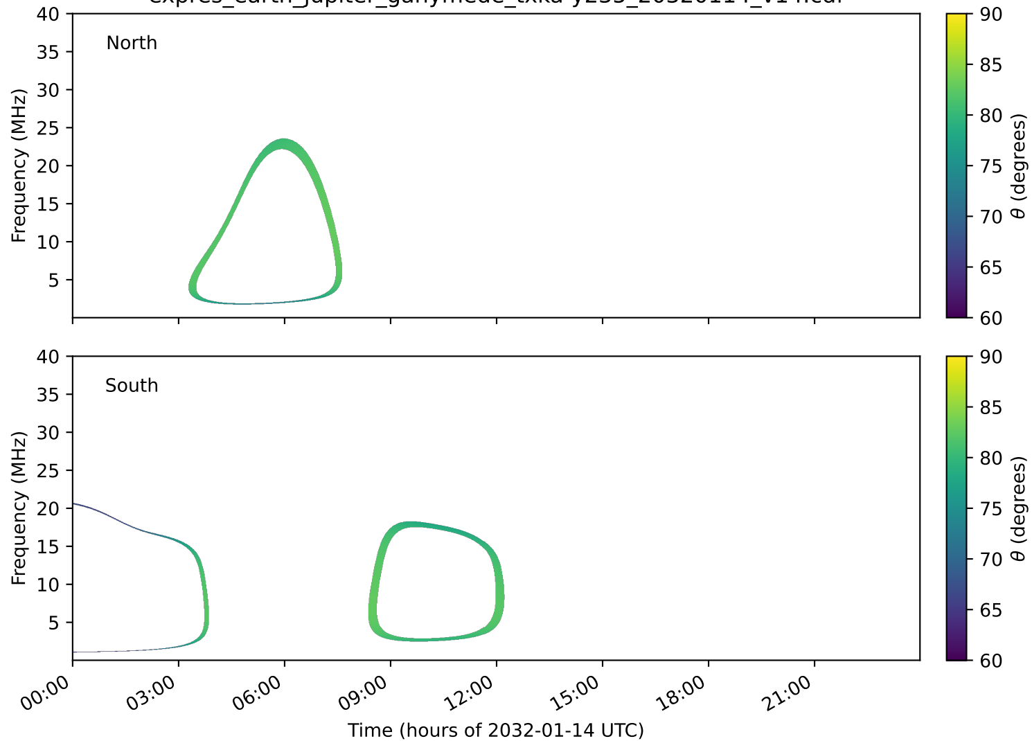
expres_earth_jupiter_ganymede_txka-y235_20320114_v14.cdf
