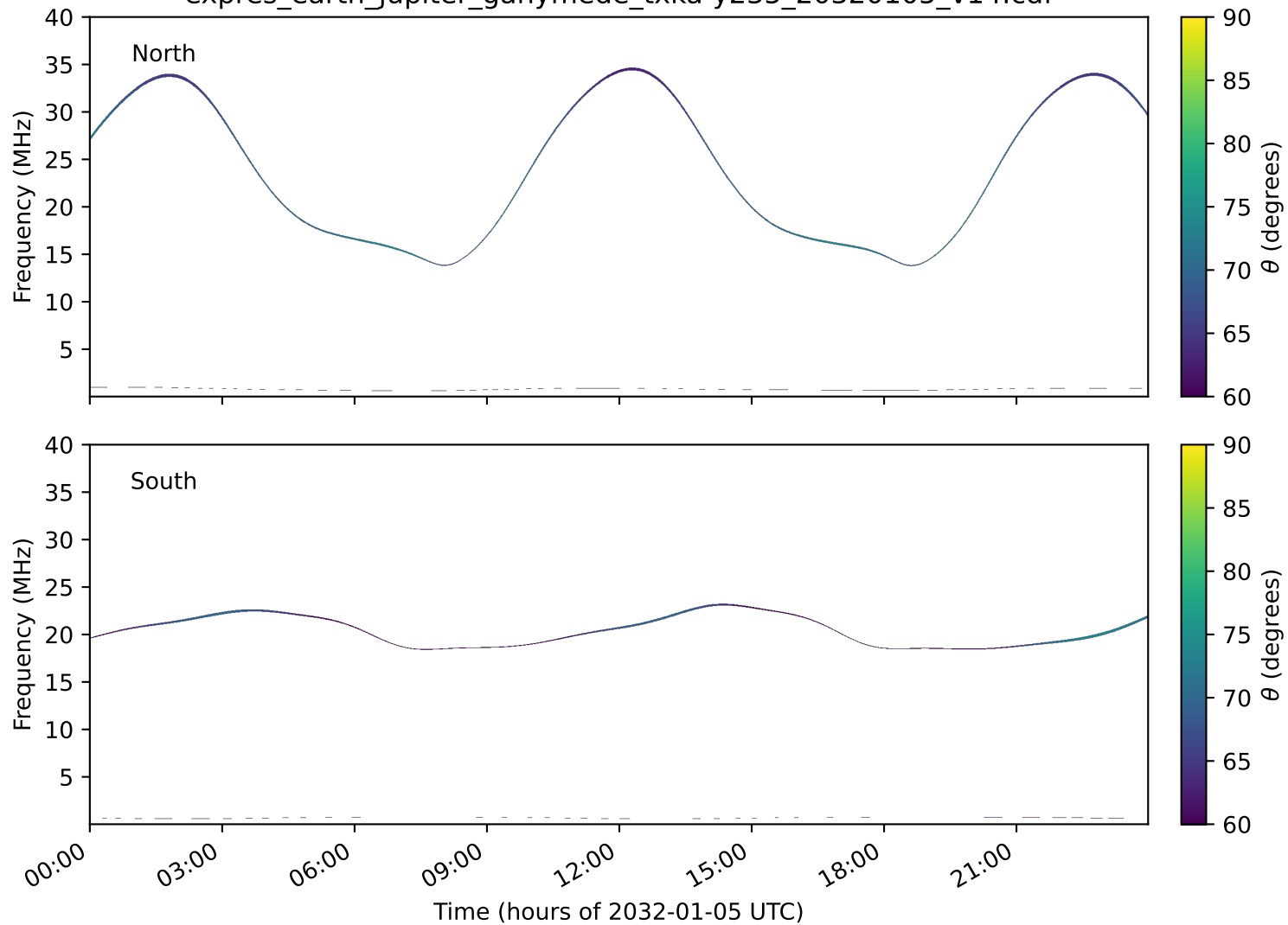
expres_earth_jupiter_ganymede_txka-y235_20320105_v14.cdf
