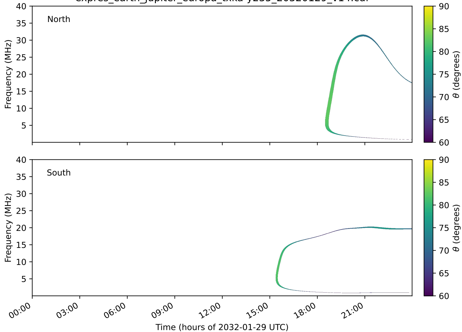
expres_earth_jupiter_europa_txka-y235_20320129_v14.cdf
