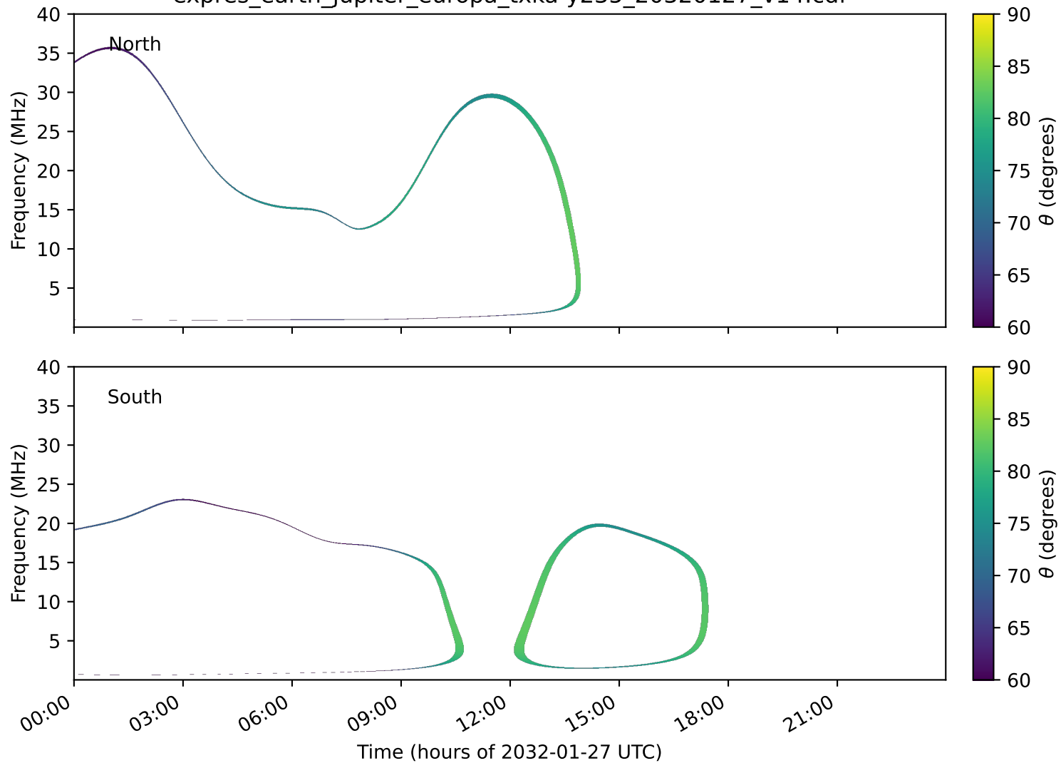
expres_earth_jupiter_europa_txka-y235_20320127_v14.cdf
