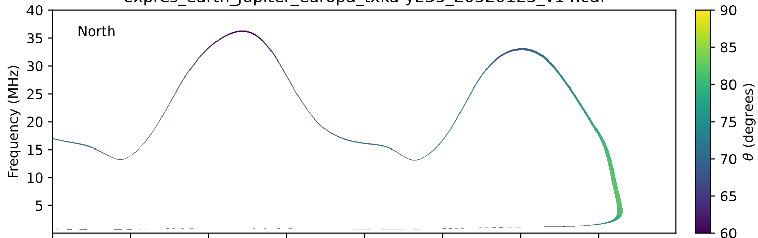
expres_earth_jupiter_europa_txka-y235_20320123_v14.cdf
