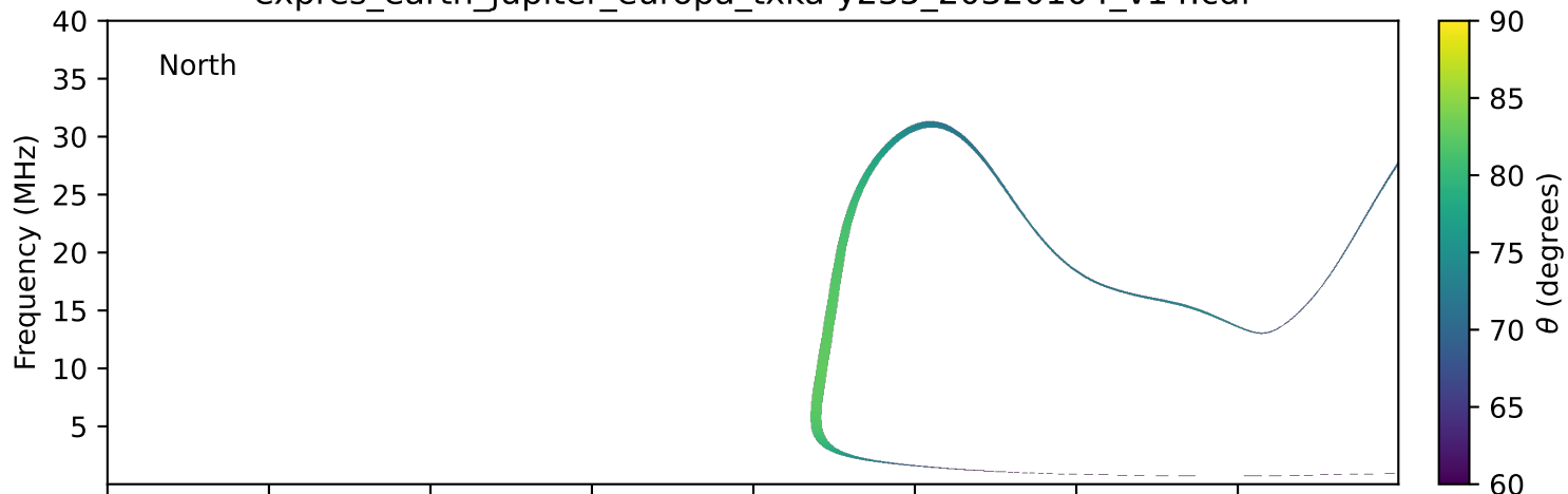
expres_earth_jupiter_europa_txka-y235_20320104_v14.cdf
