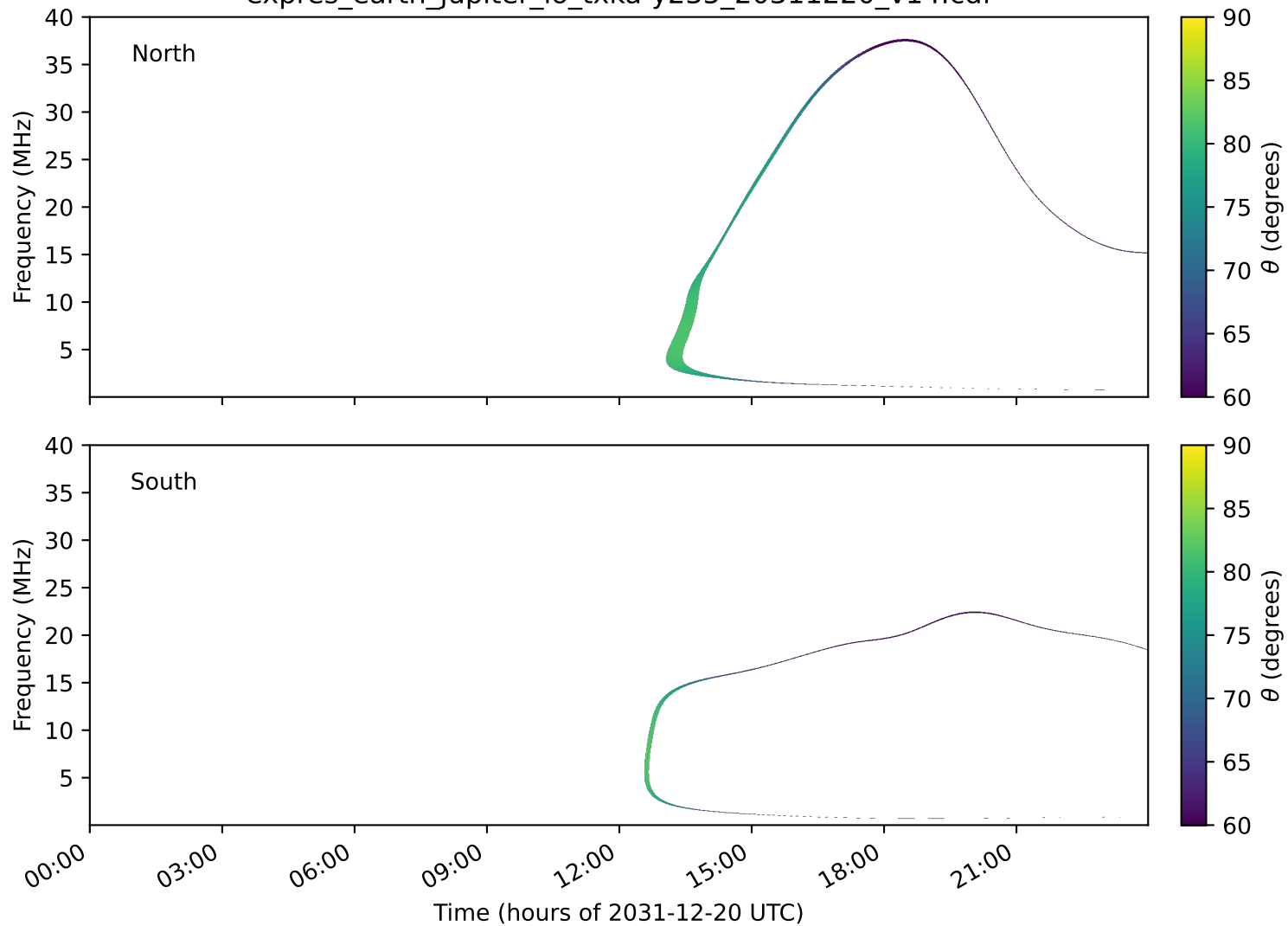
expres_earth_jupiter_io_txka-y235_20311220_v14.cdf
