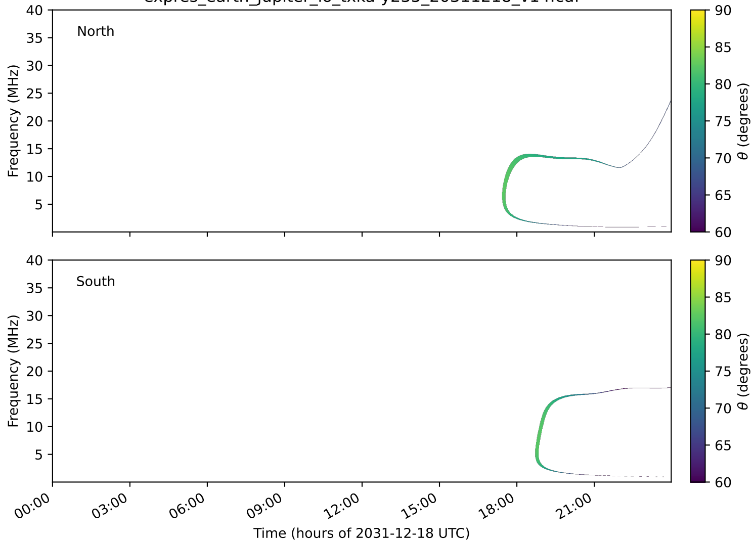
expres_earth_jupiter_io_txka-y235_20311218_v14.cdf
