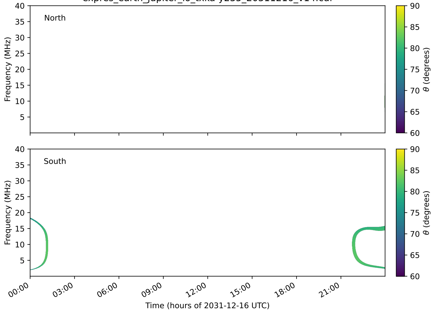
expres_earth_jupiter_io_txka-y235_20311216_v14.cdf
