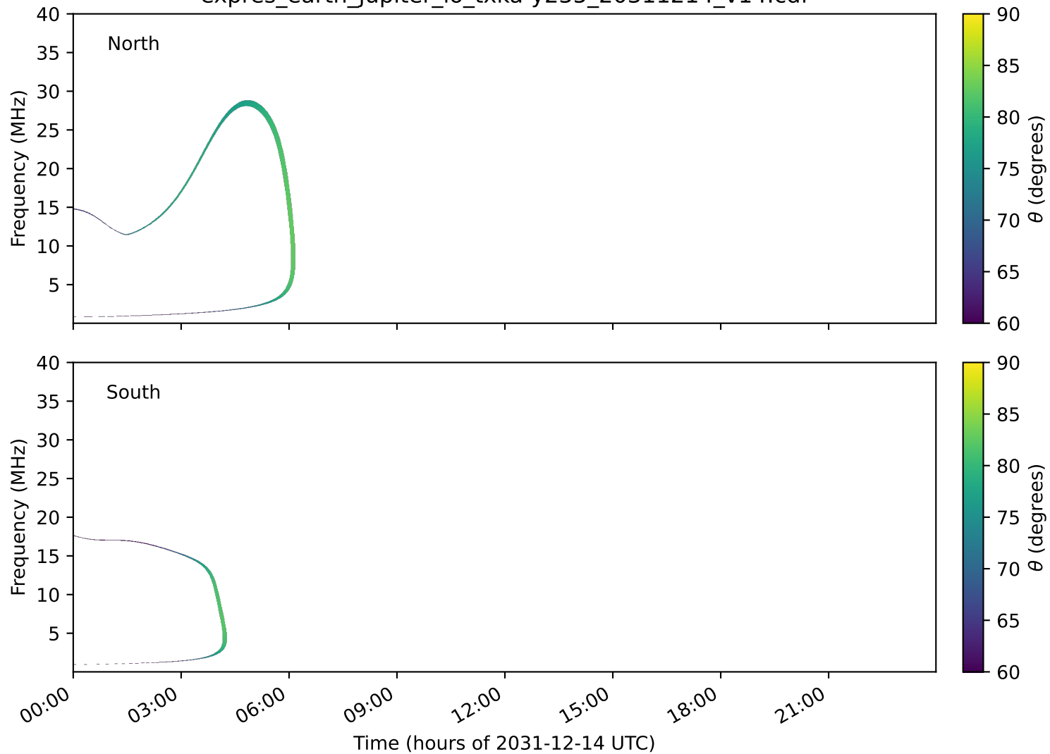
expres_earth_jupiter_io_txka-y235_20311214_v14.cdf
