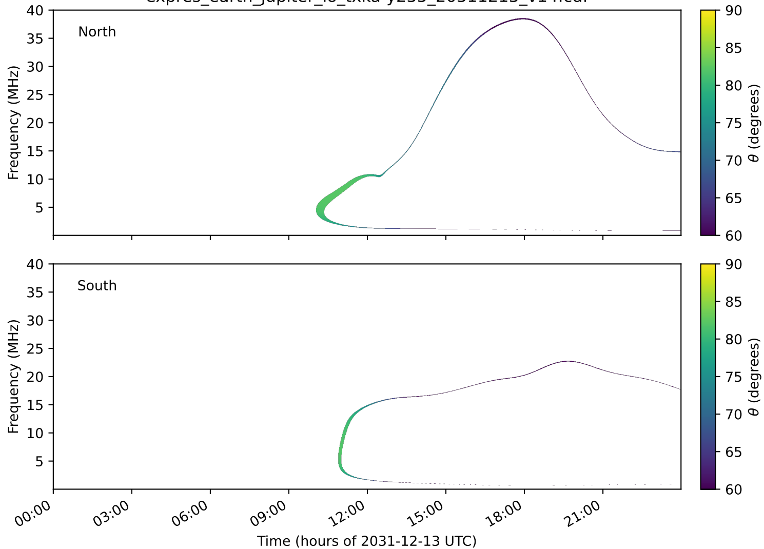
expres_earth_jupiter_io_txka-y235_20311213_v14.cdf
