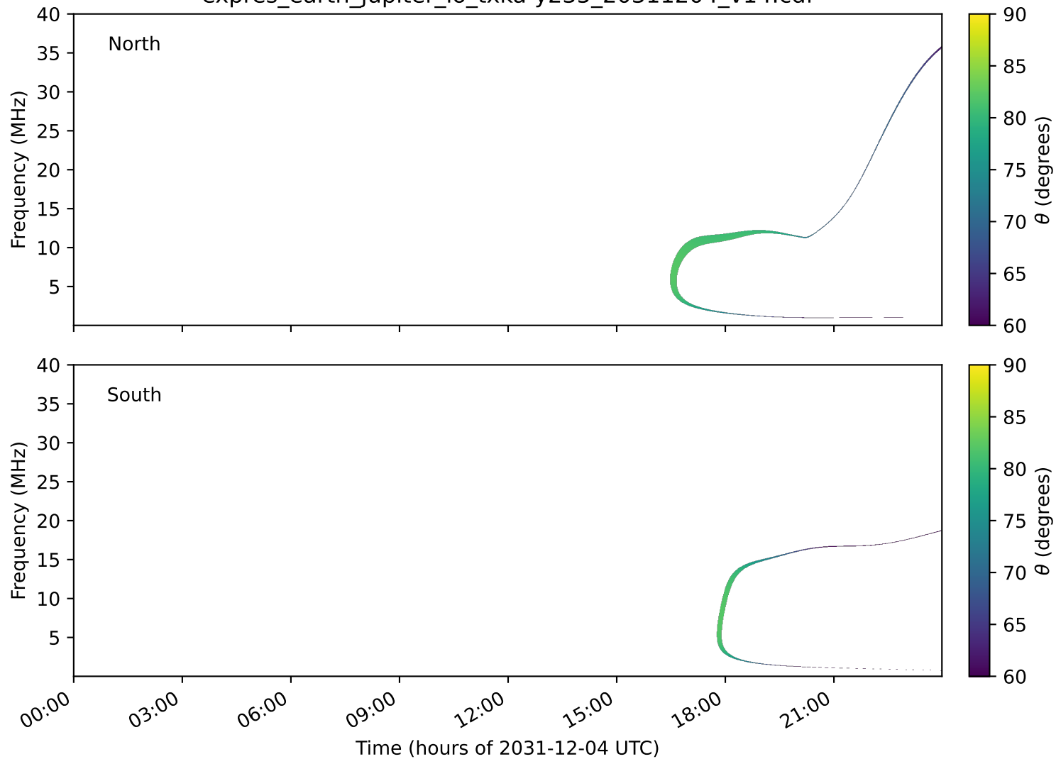
expres_earth_jupiter_io_txka-y235_20311204_v14.cdf
