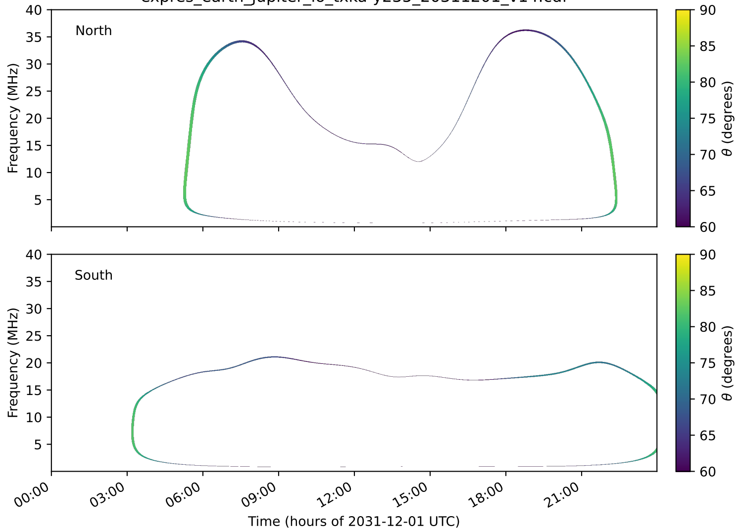
expres_earth_jupiter_io_txka-y235_20311201_v14.cdf
