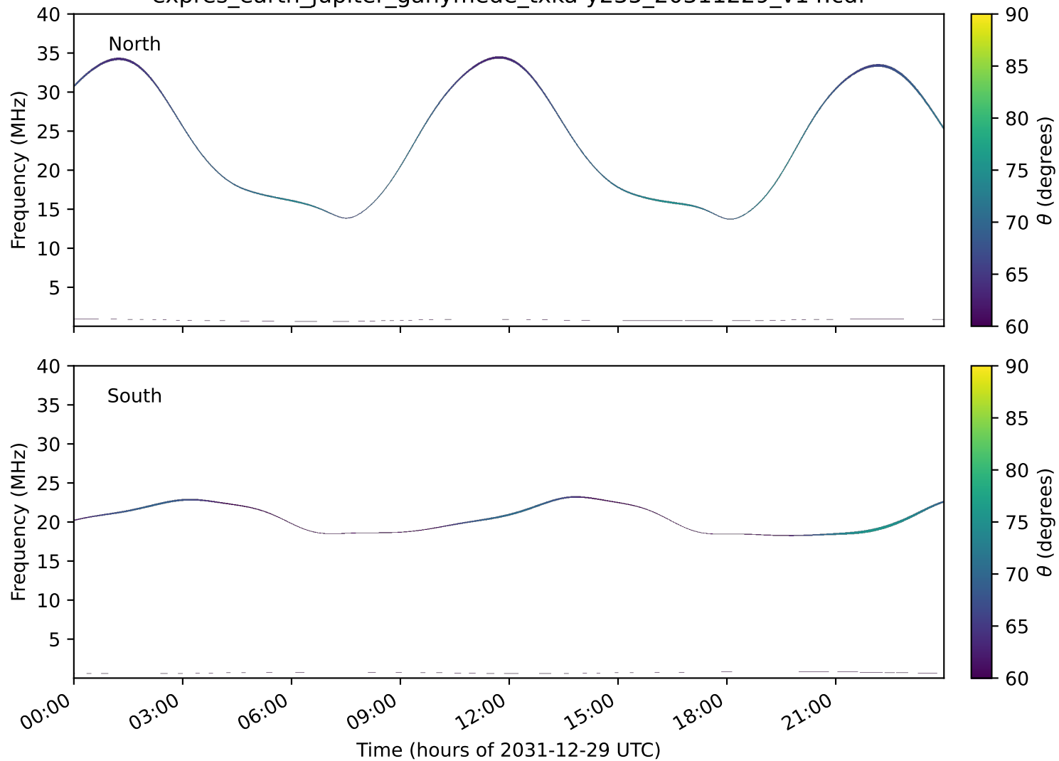
expres_earth_jupiter_ganymede_txka-y235_20311229_v14.cdf
