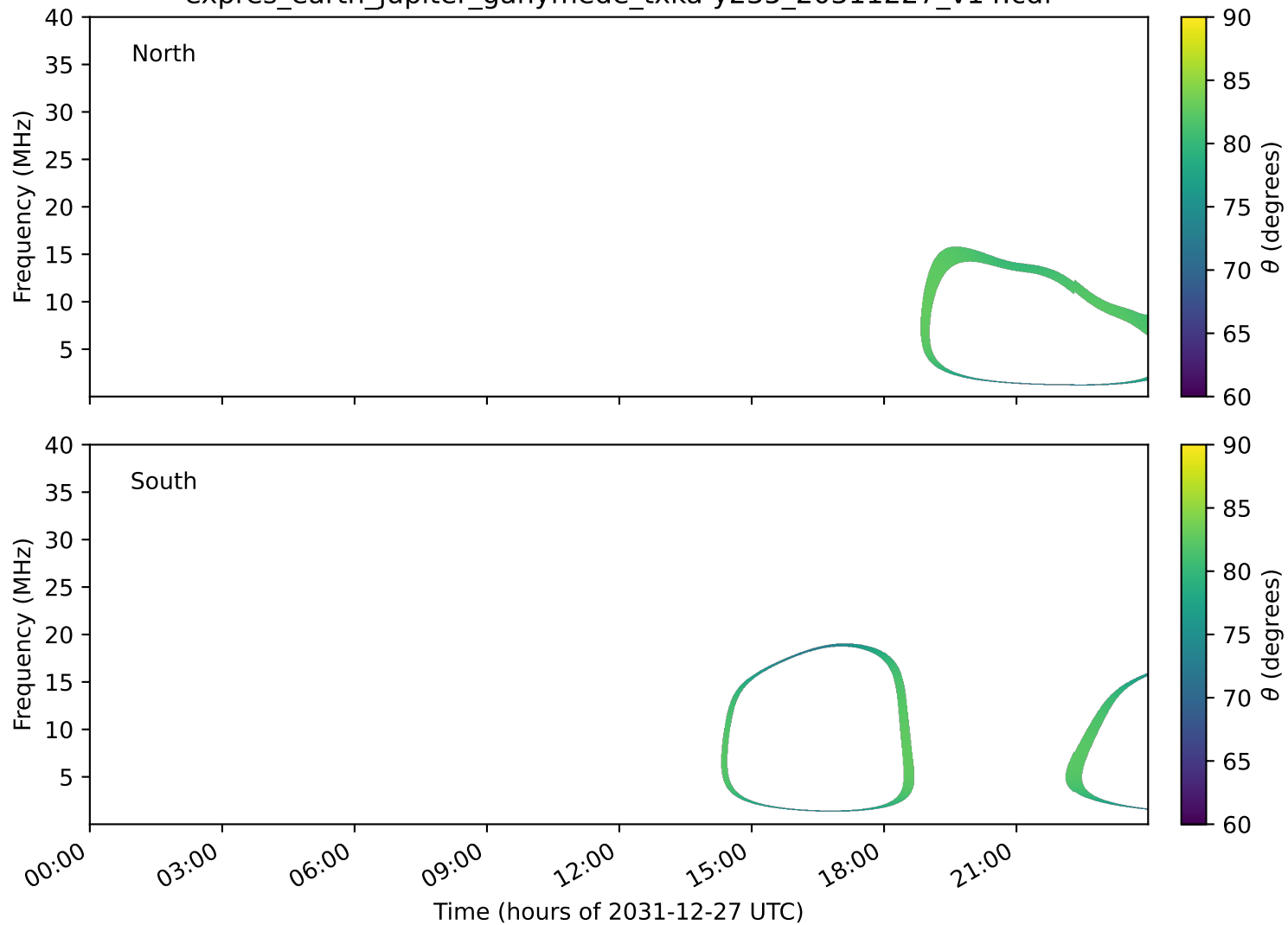
expres_earth_jupiter_ganymede_txka-y235_20311227_v14.cdf
