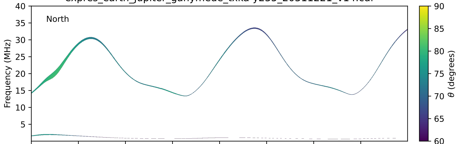
expres_earth_jupiter_ganymede_txka-y235_20311221_v14.cdf
