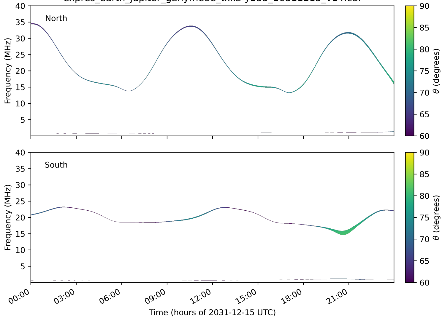
expres_earth_jupiter_ganymede_txka-y235_20311215_v14.cdf
