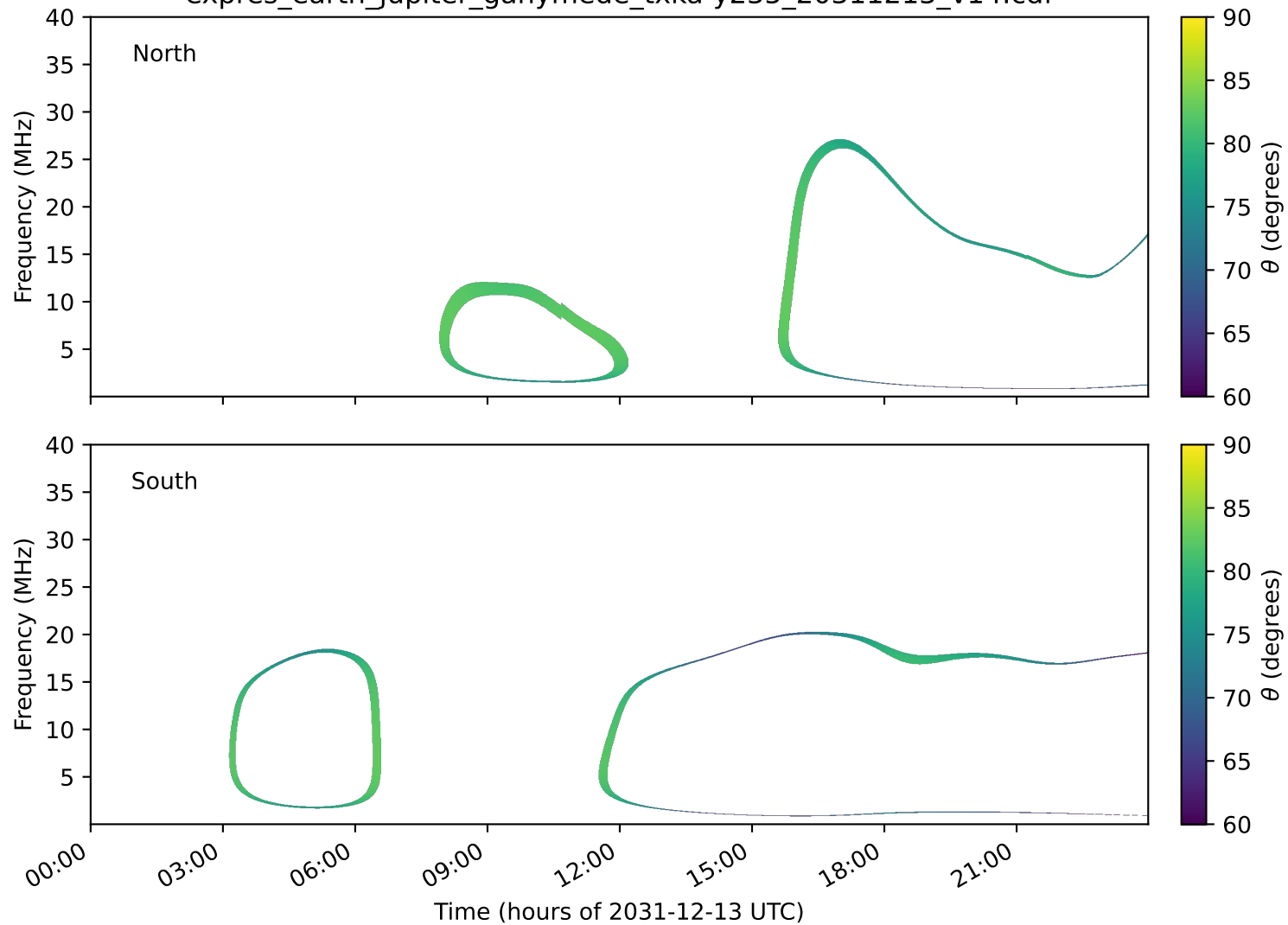
expres_earth_jupiter_ganymede_txka-y235_20311213_v14.cdf
