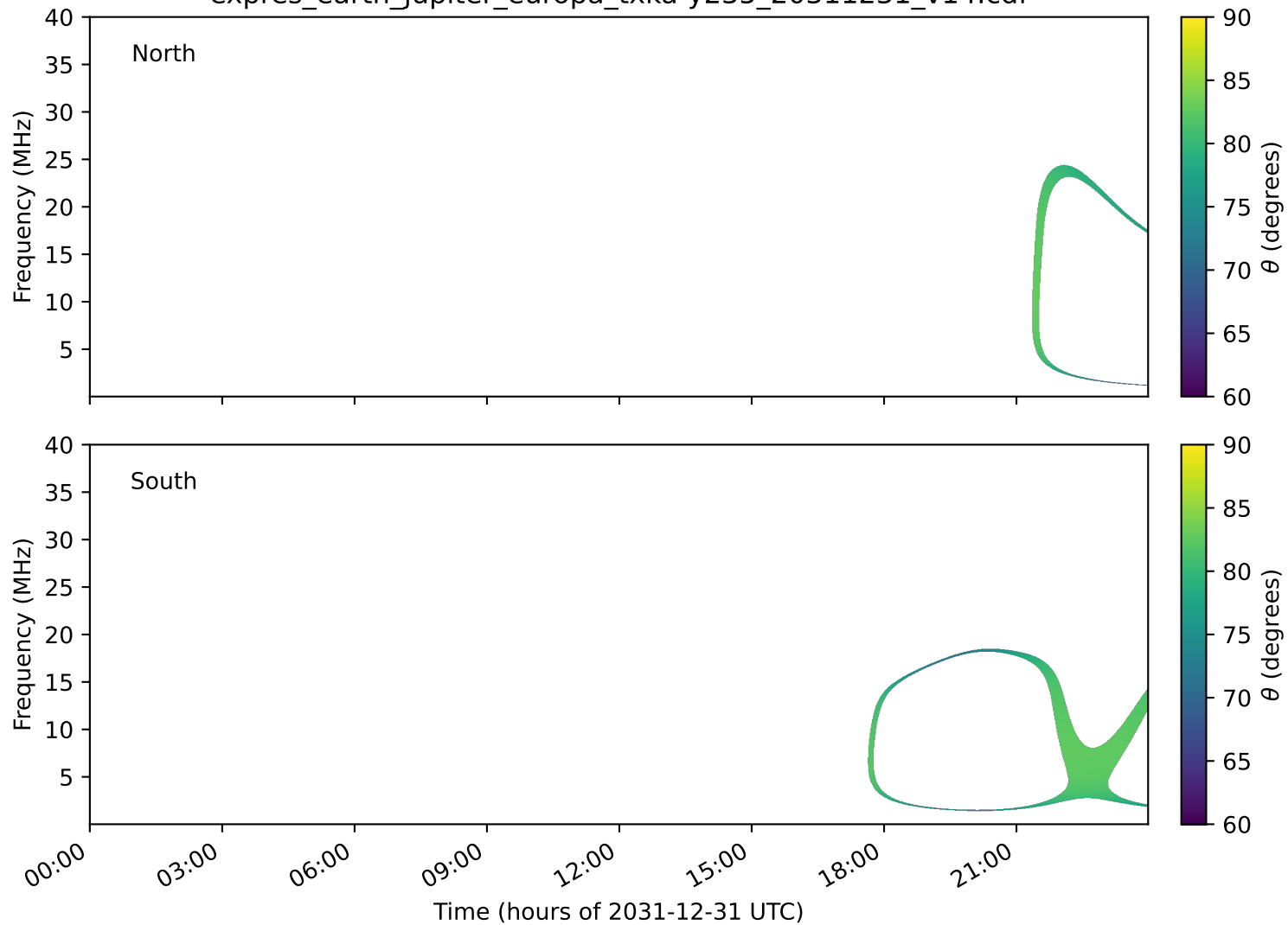
expres_earth_jupiter_europa_txka-y235_20311231_v14.cdf
