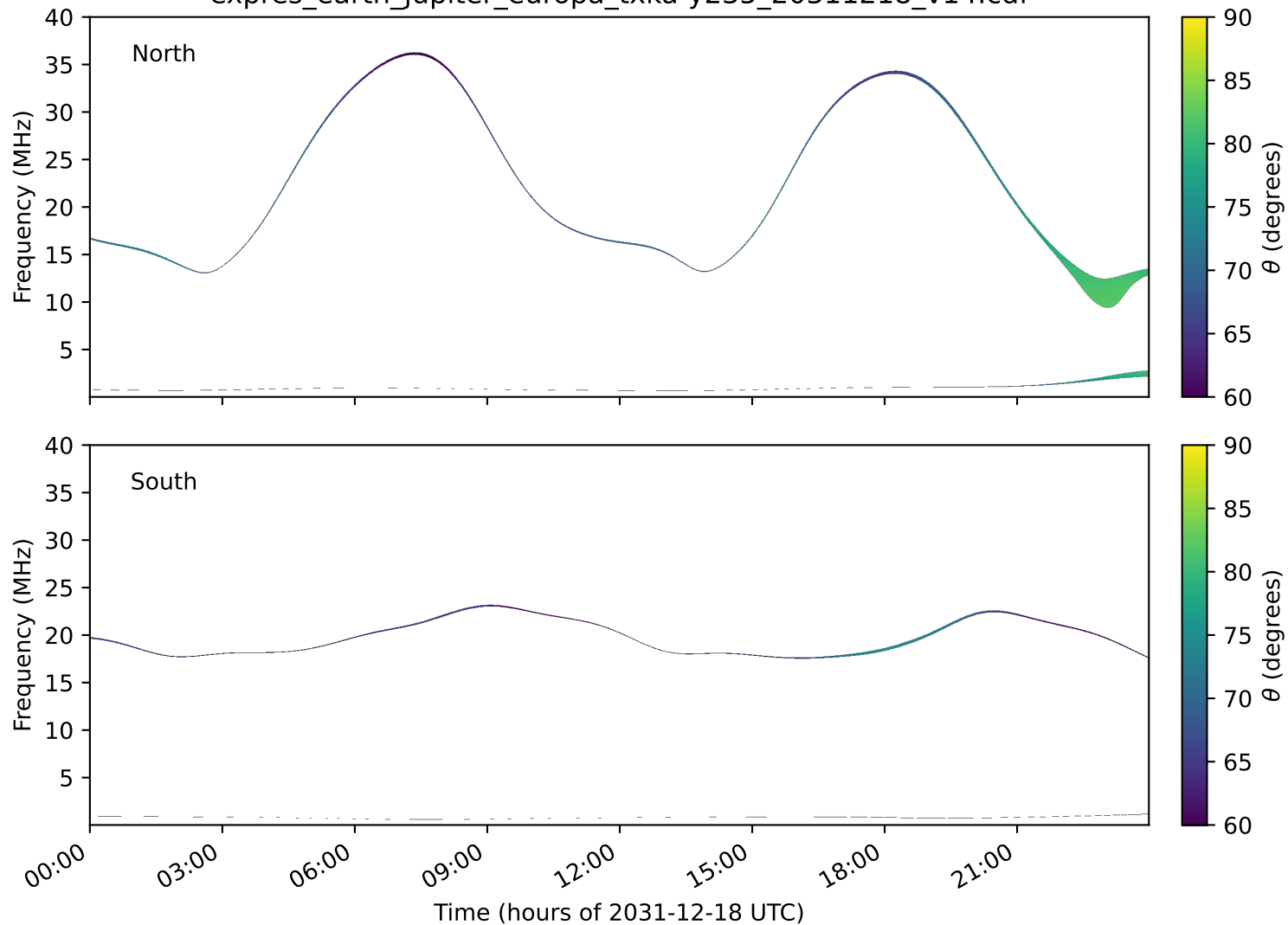
expres_earth_jupiter_europa_txka-y235_20311218_v14.cdf
