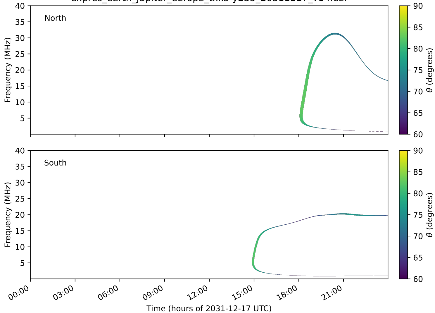
expres_earth_jupiter_europa_txka-y235_20311217_v14.cdf
