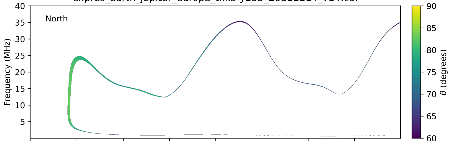
expres_earth_jupiter_europa_txka-y235_20311214_v14.cdf
