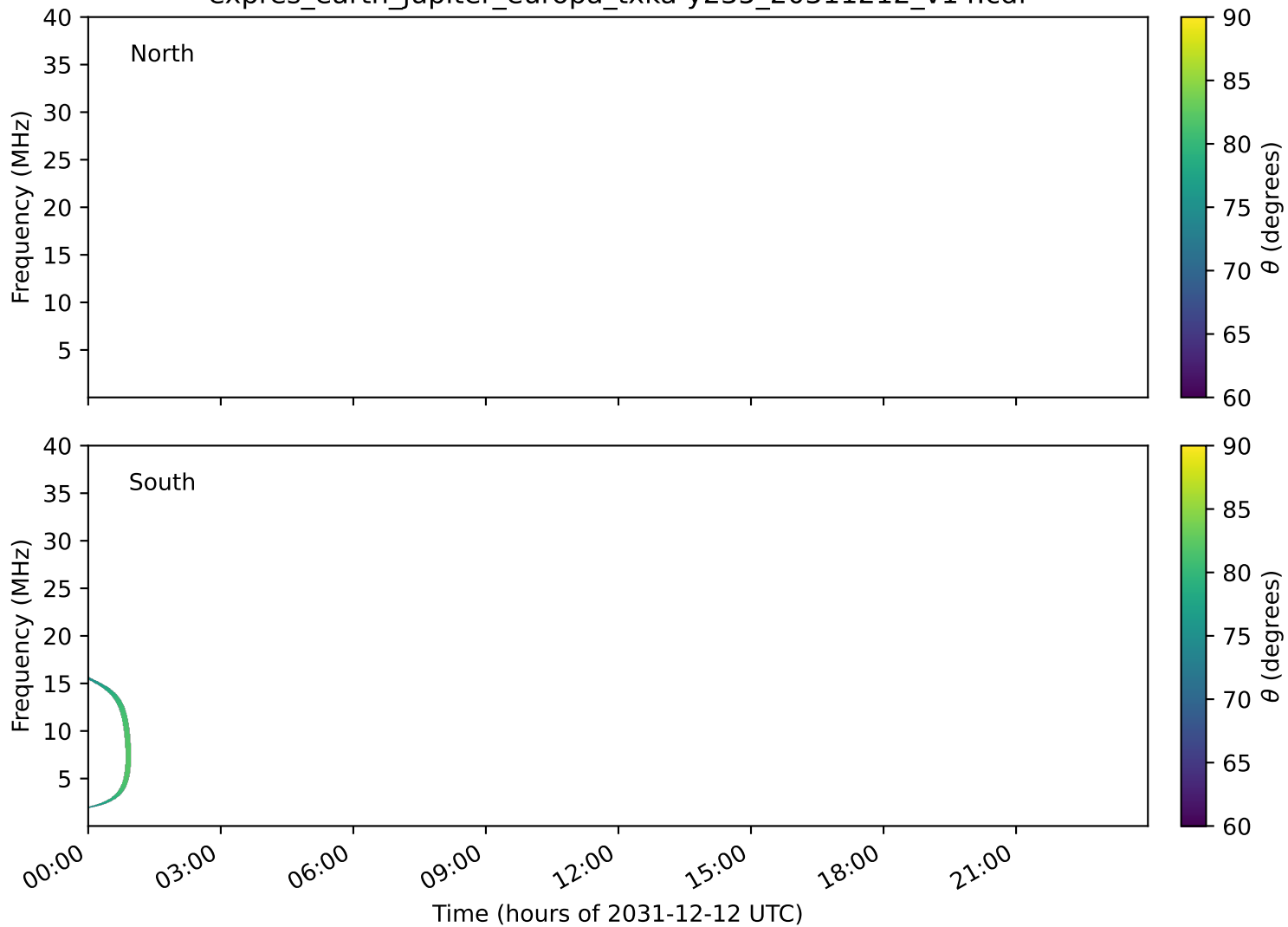
expres_earth_jupiter_europa_txka-y235_20311212_v14.cdf
